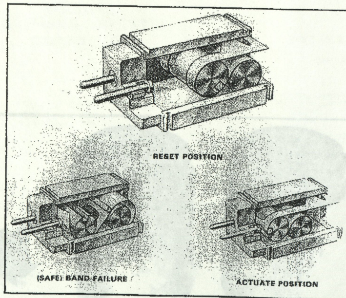
Figure 21. MC4146/MC4147 Rolamites
